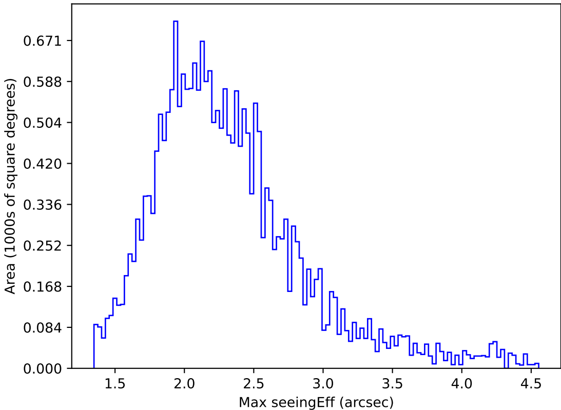
too_elab_r32_d3_griz_v3.4_10yrs All sky y band: Max seeingEff
