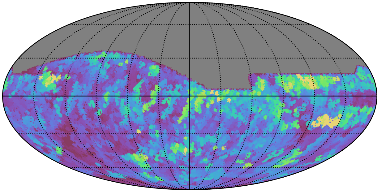
too_elab_r32_d3_griz_v3.4_10yrs All sky r band: Max seeingEff
