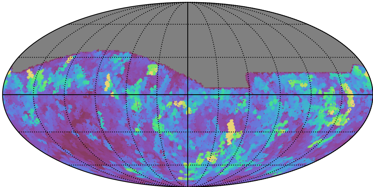
too_elab_r32_d3_griz_v3.4_10yrs All sky i band: Max seeingEff
