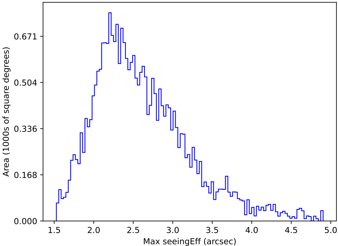
too_elab_r32_d3_griz_v3.4_10yrs All sky i band: Max seeingEff
