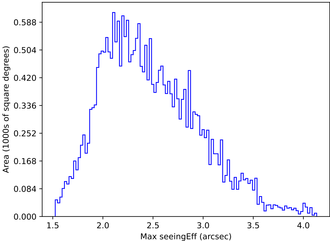
too_elab_r32_d3_griz_v3.4_10yrs All sky g band: Max seeingEff
