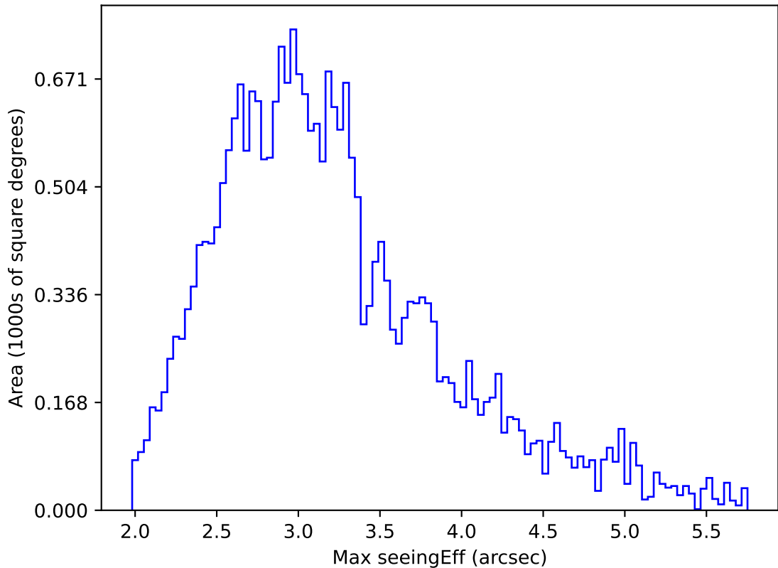
too_elab_r32_d3_griz_v3.4_10yrs All sky all bands: Max seeingEff
