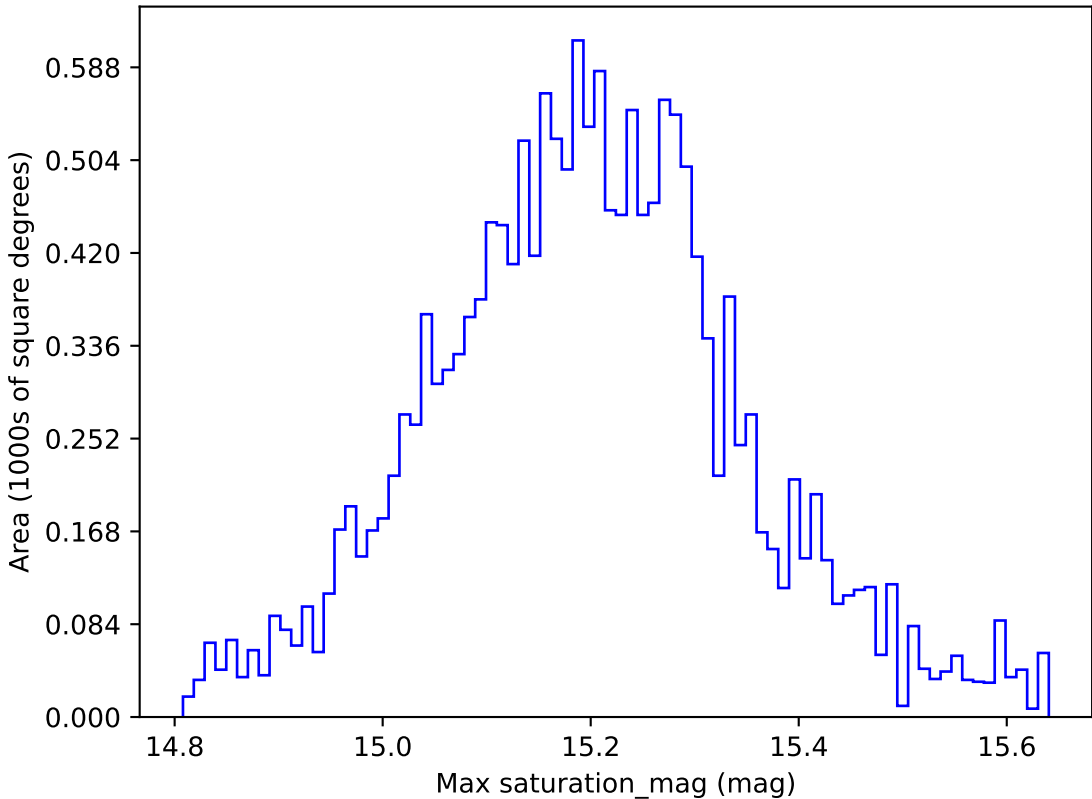
too_elab_r32_d3_griz_v3.4_10yrs WFD z band: Max saturation_mag
