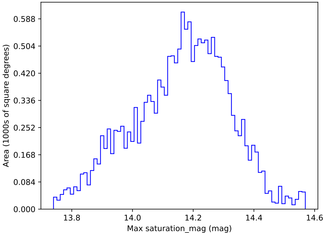
too_elab_r32_d3_griz_v3.4_10yrs WFD y band: Max saturation_mag
