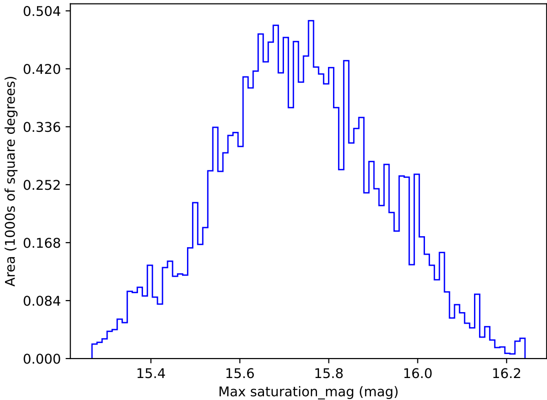
too_elab_r32_d3_griz_v3.4_10yrs WFD g band: Max saturation_mag
