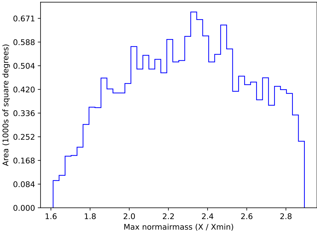
too_elab_r32_d3_griz_v3.4_10yrs WFD z band: Max normairmass
