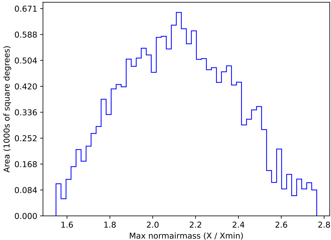
too_elab_r32_d3_griz_v3.4_10yrs WFD y band: Max normairmass
