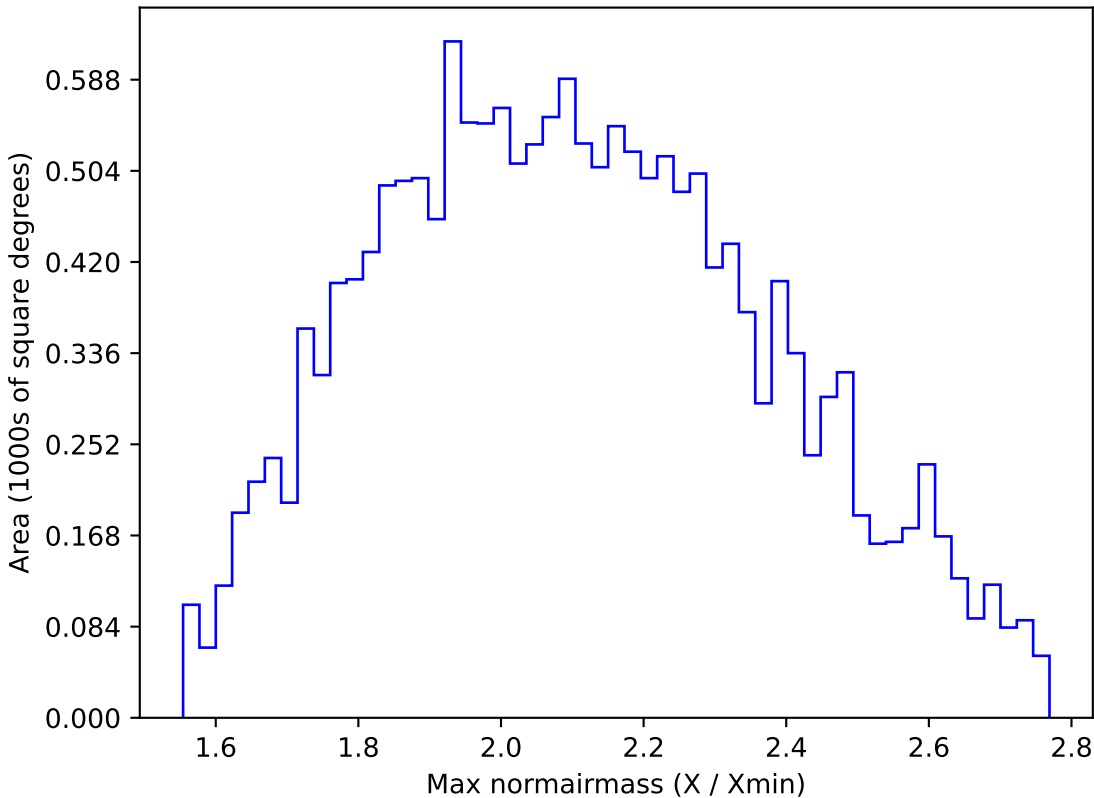
too_elab_r32_d3_griz_v3.4_10yrs WFD y band: Max normairmass
