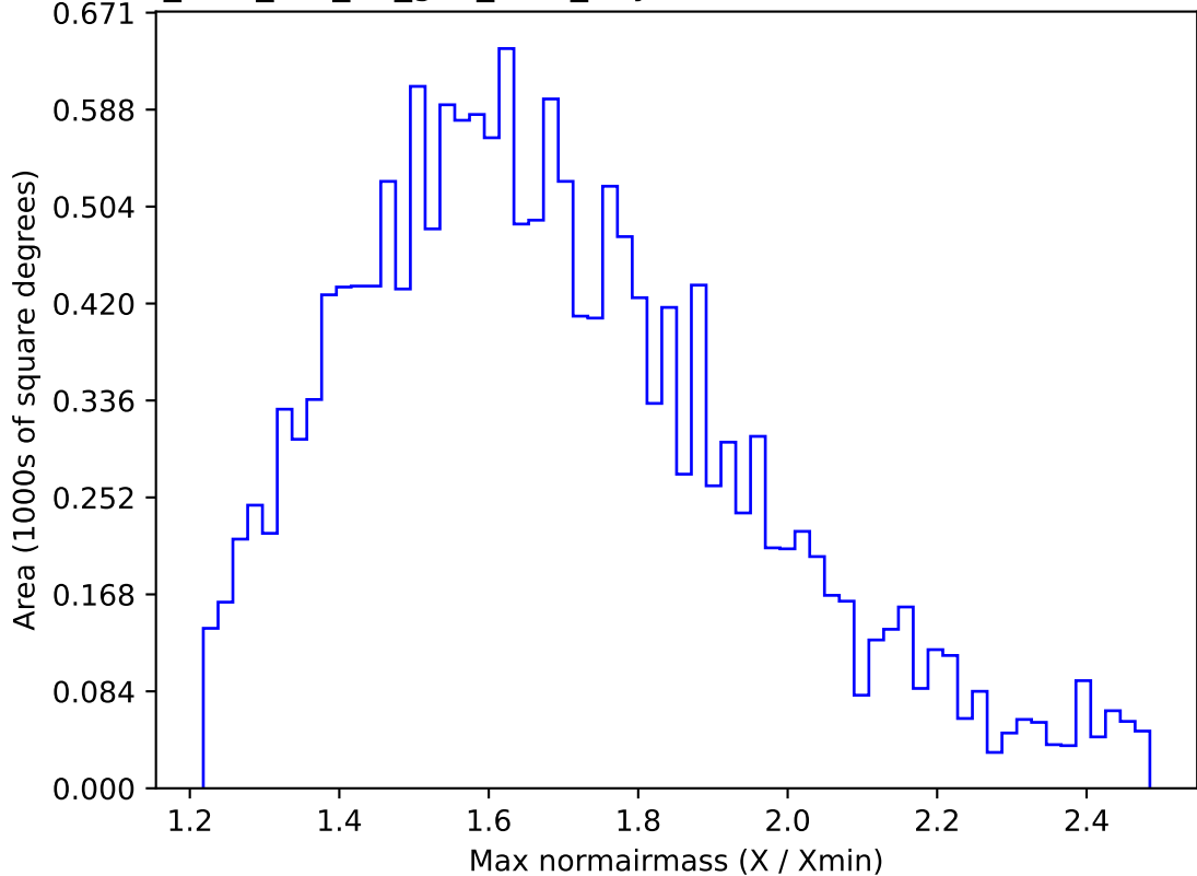
too_elab_r32_d3_griz_v3.4_10yrs WFD u band: Max normairmass
