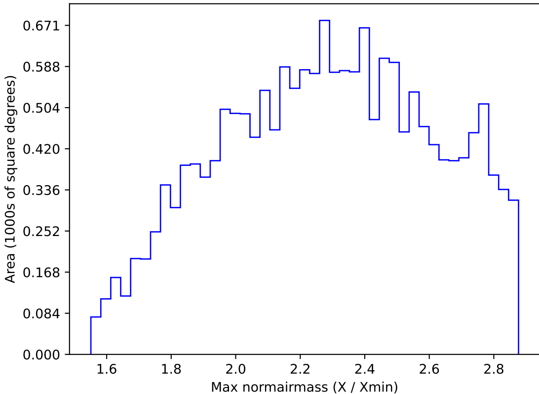
too_elab_r32_d3_griz_v3.4_10yrs WFD i band: Max normairmass
