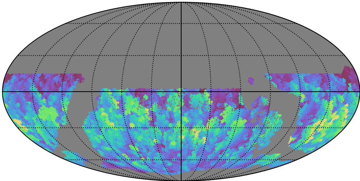
too_elab_r32_d3_griz_v3.4_10yrs WFD g band: Max normairmass
