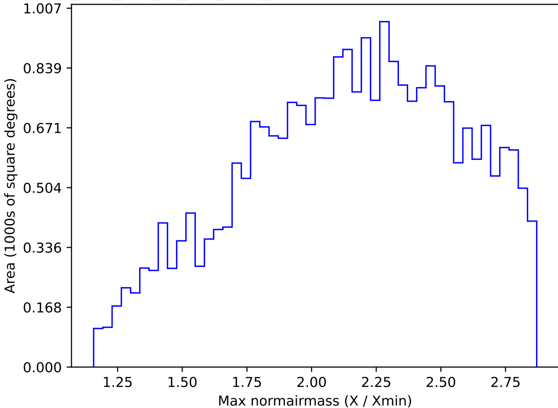
too_elab_r32_d3_griz_v3.4_10yrs All sky i band: Max normairmass
