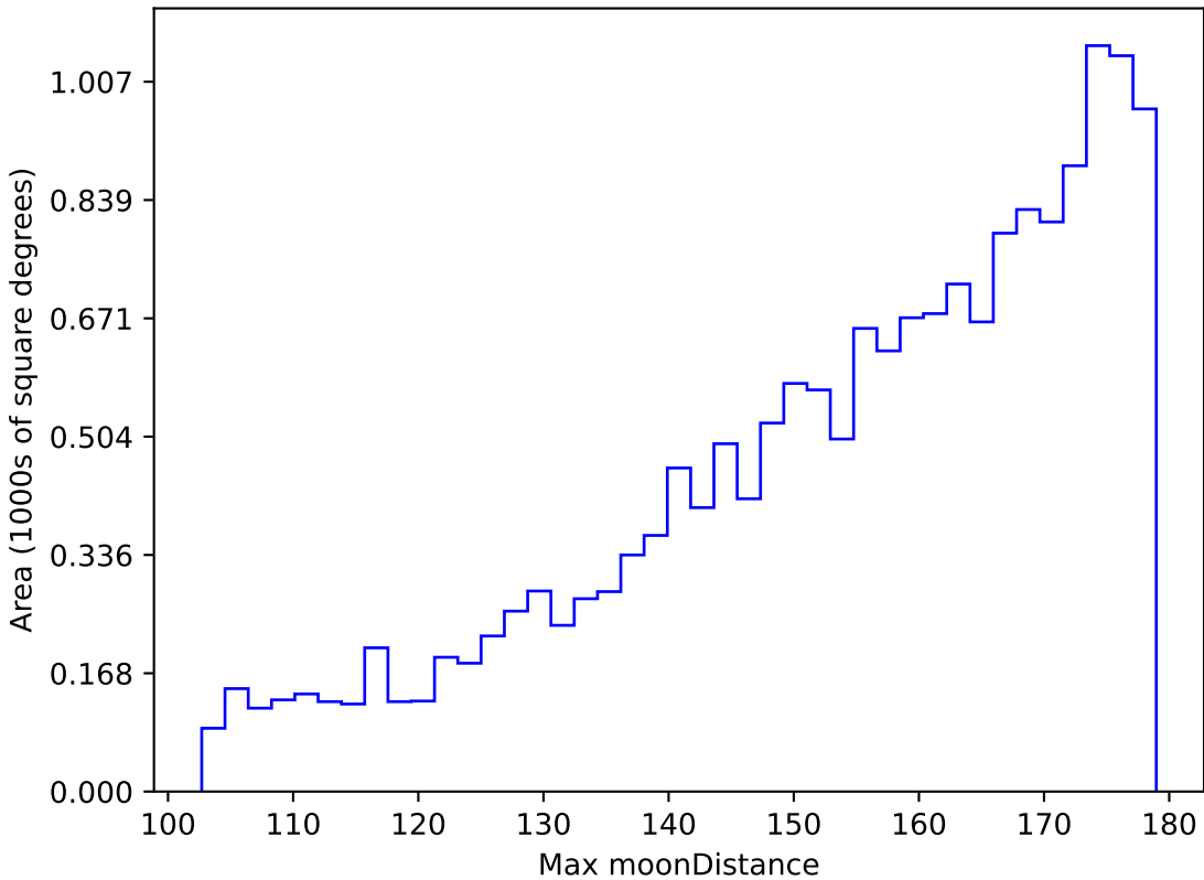
too_elab_r32_d3_griz_v3.4_10yrs WFD z band: Max moonDistance
