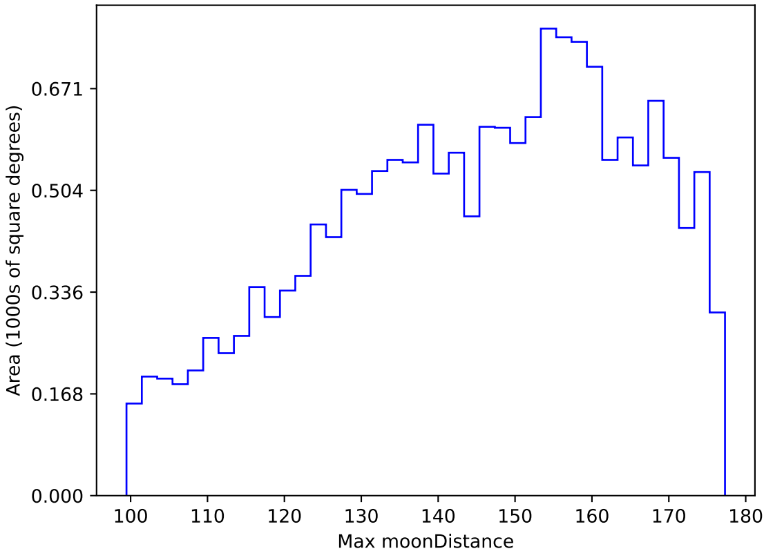
too_elab_r32_d3_griz_v3.4_10yrs WFD y band: Max moonDistance
