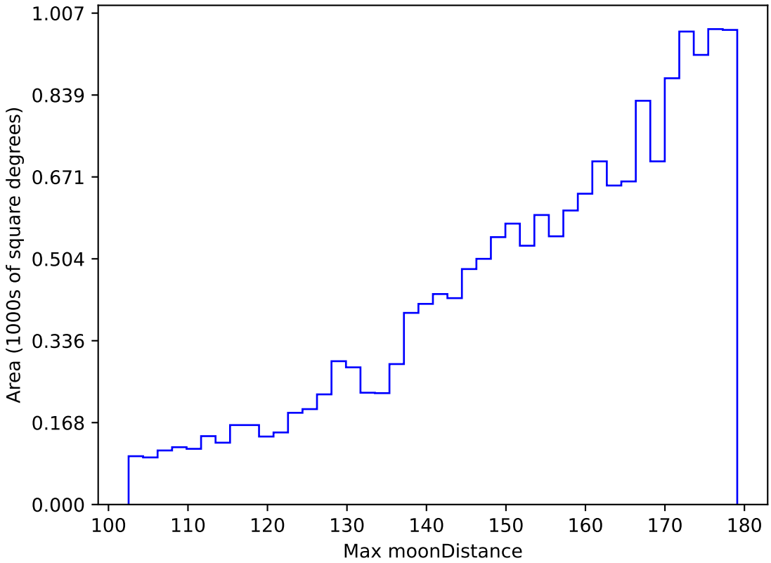
too_elab_r32_d3_griz_v3.4_10yrs WFD u band: Max moonDistance
