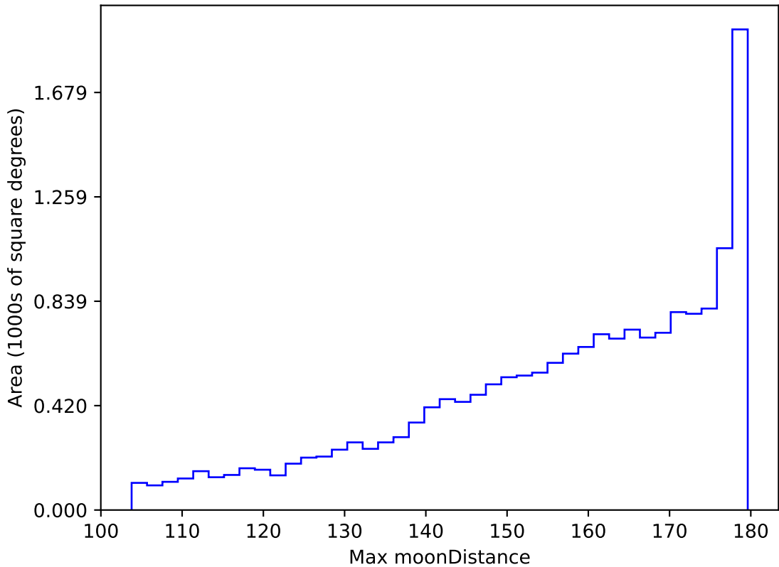
too_elab_r32_d3_griz_v3.4_10yrs WFD all bands: Max moonDistance
