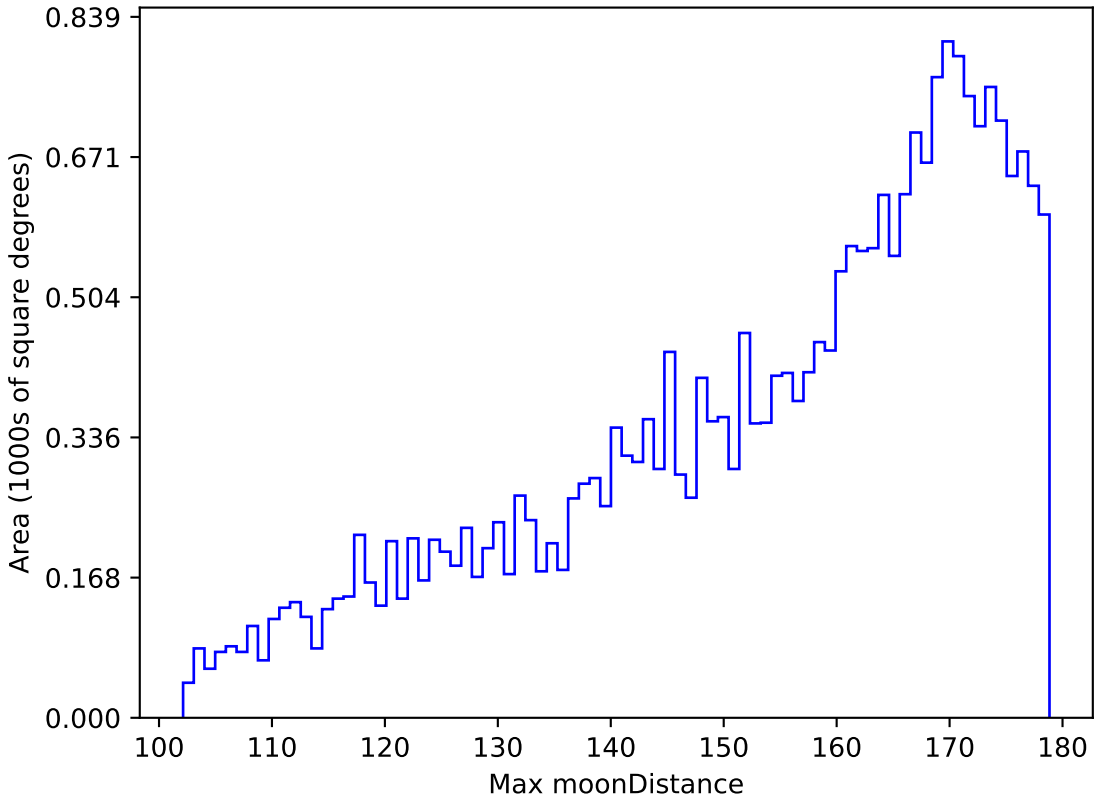
too_elab_r32_d3_griz_v3.4_10yrs All sky z band: Max moonDistance
