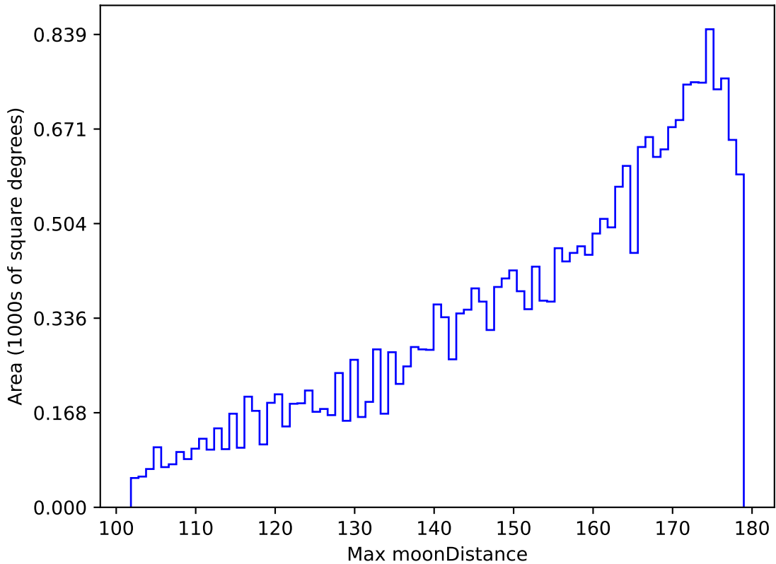
too_elab_r32_d3_griz_v3.4_10yrs All sky z band: Max moonDistance
