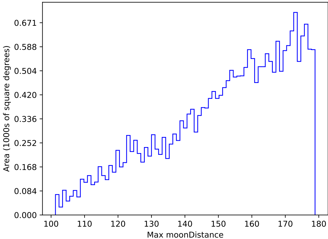
too_elab_r32_d3_griz_v3.4_10yrs All sky u band: Max moonDistance
