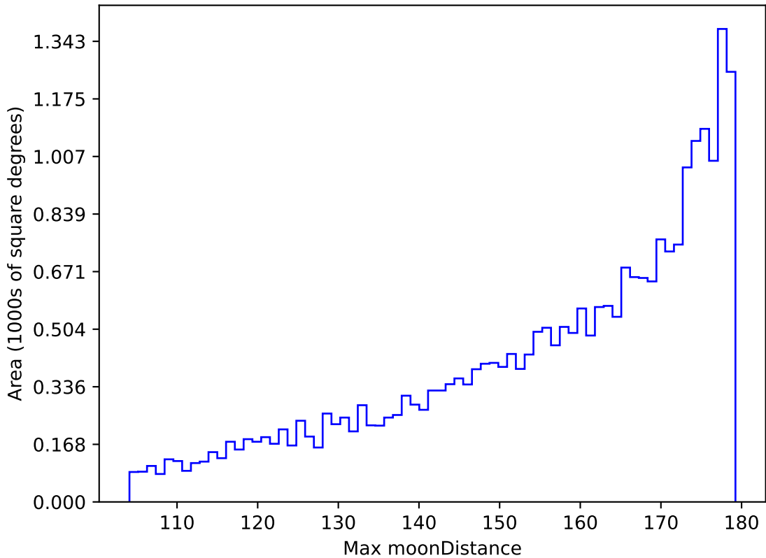
too_elab_r32_d3_griz_v3.4_10yrs All sky r band: Max moonDistance
