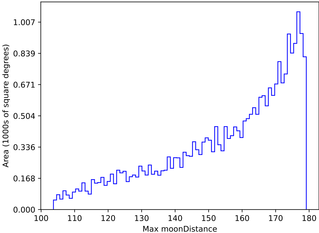
too_elab_r32_d3_griz_v3.4_10yrs All sky i band: Max moonDistance
