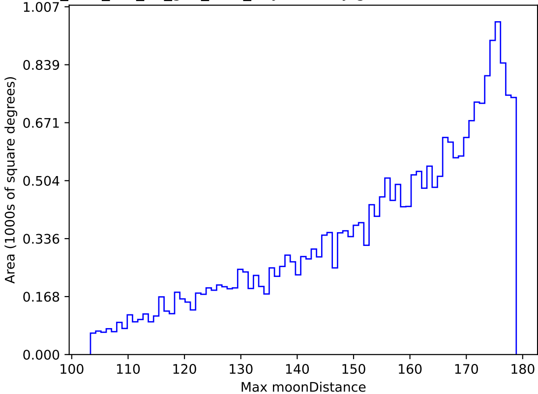
too_elab_r32_d3_griz_v3.4_10yrs All sky g band: Max moonDistance
