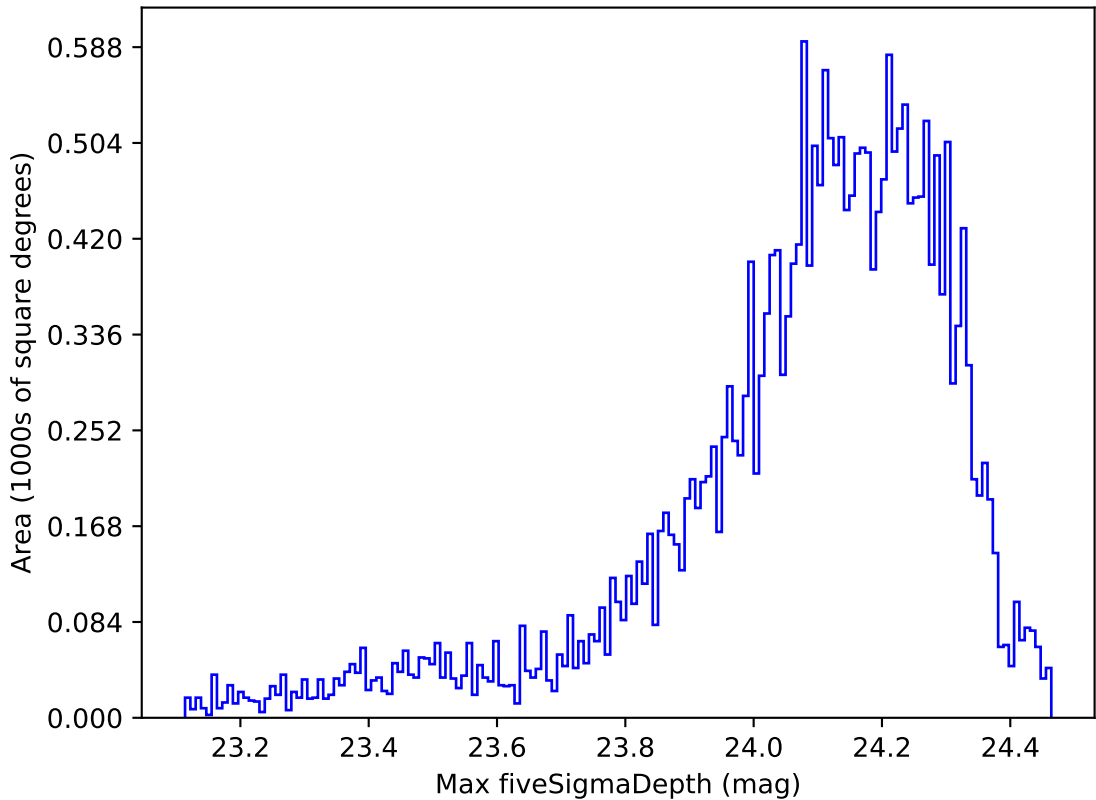
too_elab_r32_d3_griz_v3.4_10yrs Yr 1 i band: Max fiveSigmaDepth
