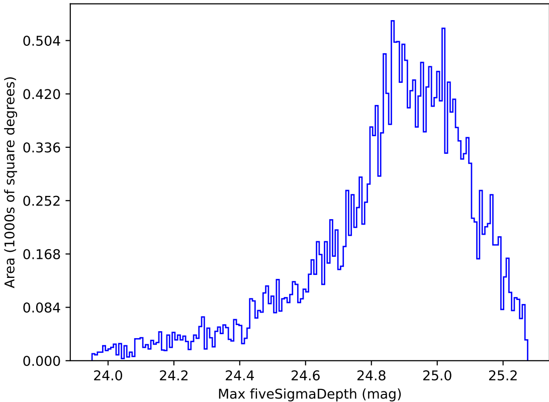
too_elab_r32_d3_griz_v3.4_10yrs Yr 1 g band: Max fiveSigmaDepth
