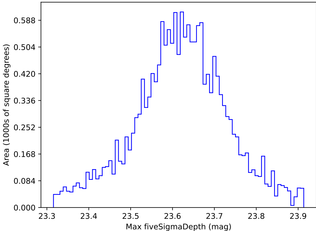
too_elab_r32_d3_griz_v3.4_10yrs WFD z band: Max fiveSigmaDepth
