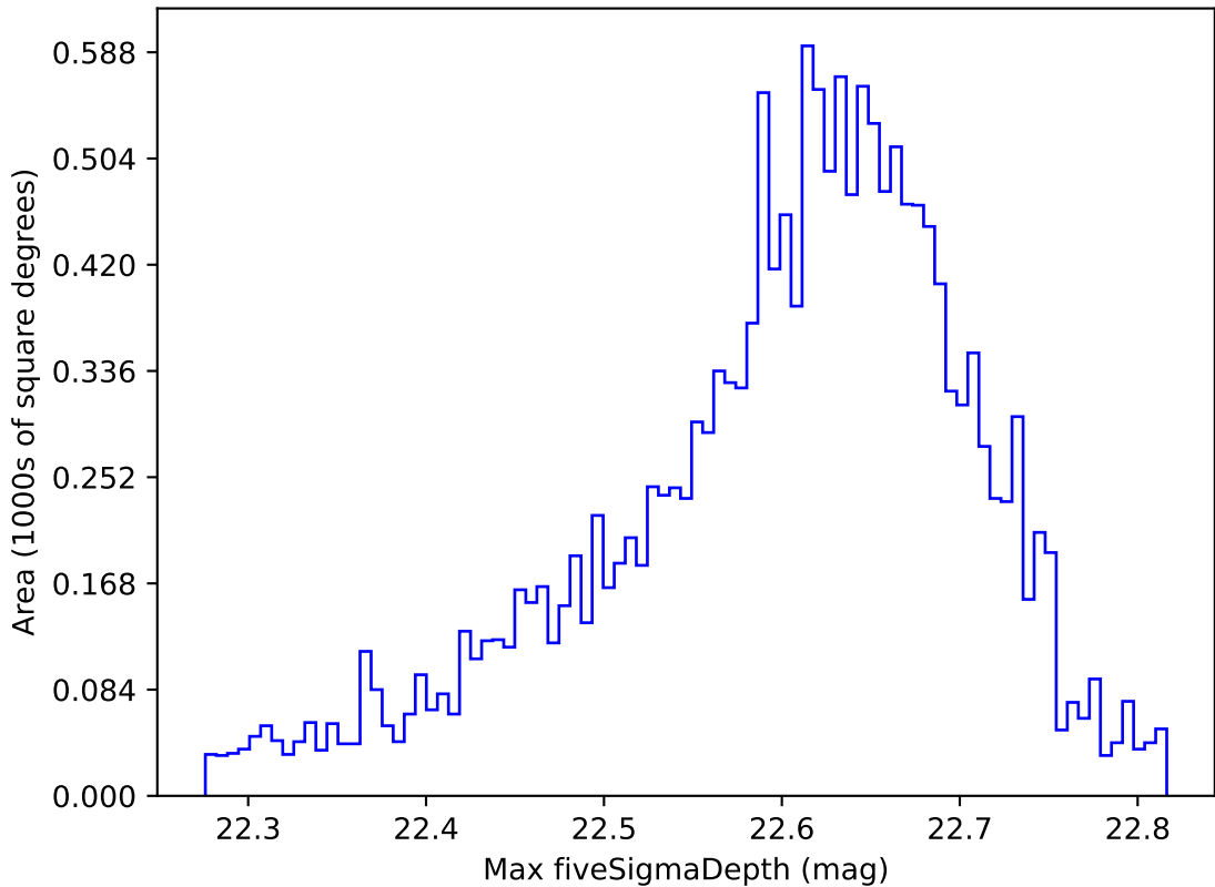
too_elab_r32_d3_griz_v3.4_10yrs WFD y band: Max fiveSigmaDepth
