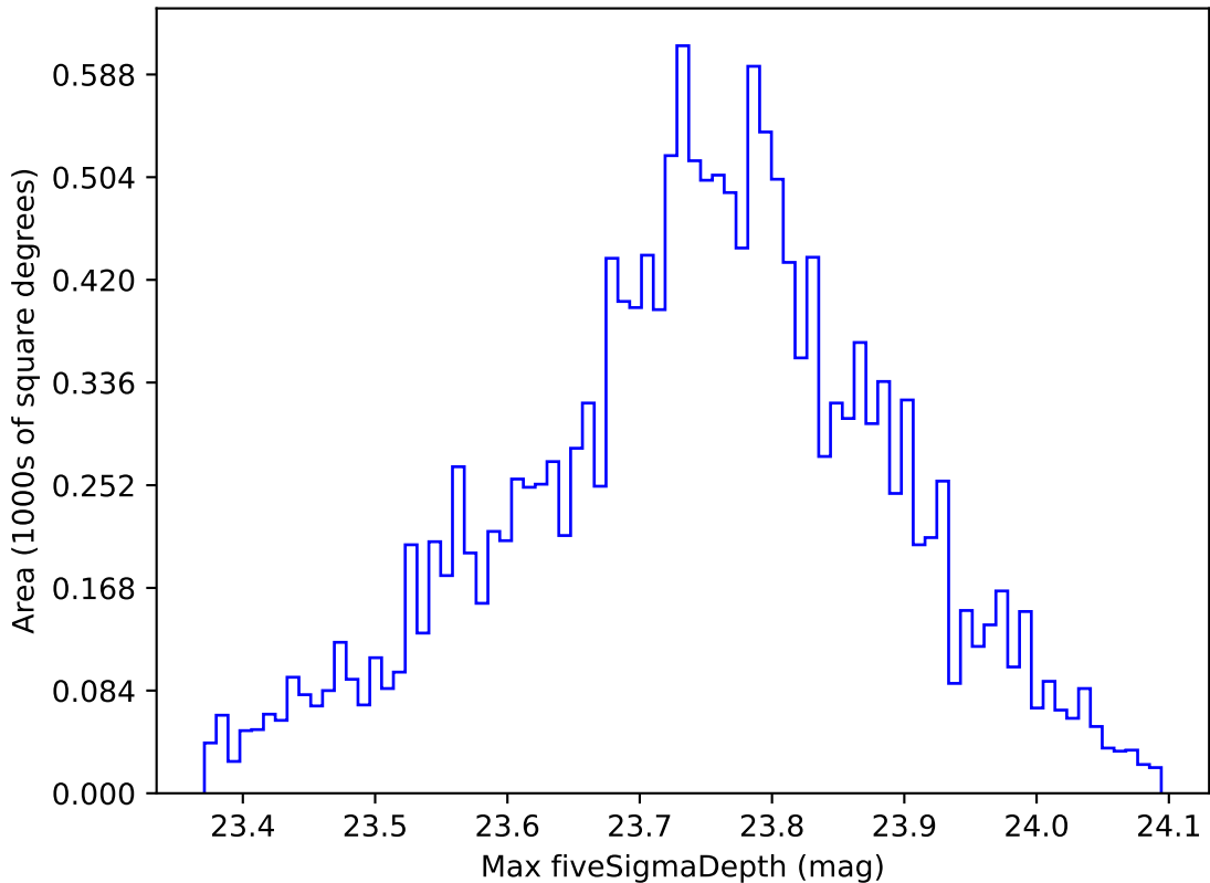
too_elab_r32_d3_griz_v3.4_10yrs WFD u band: Max fiveSigmaDepth
