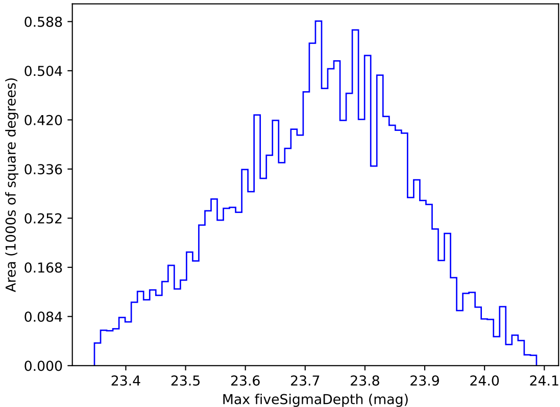
too_elab_r32_d3_griz_v3.4_10yrs WFD u band: Max fiveSigmaDepth
