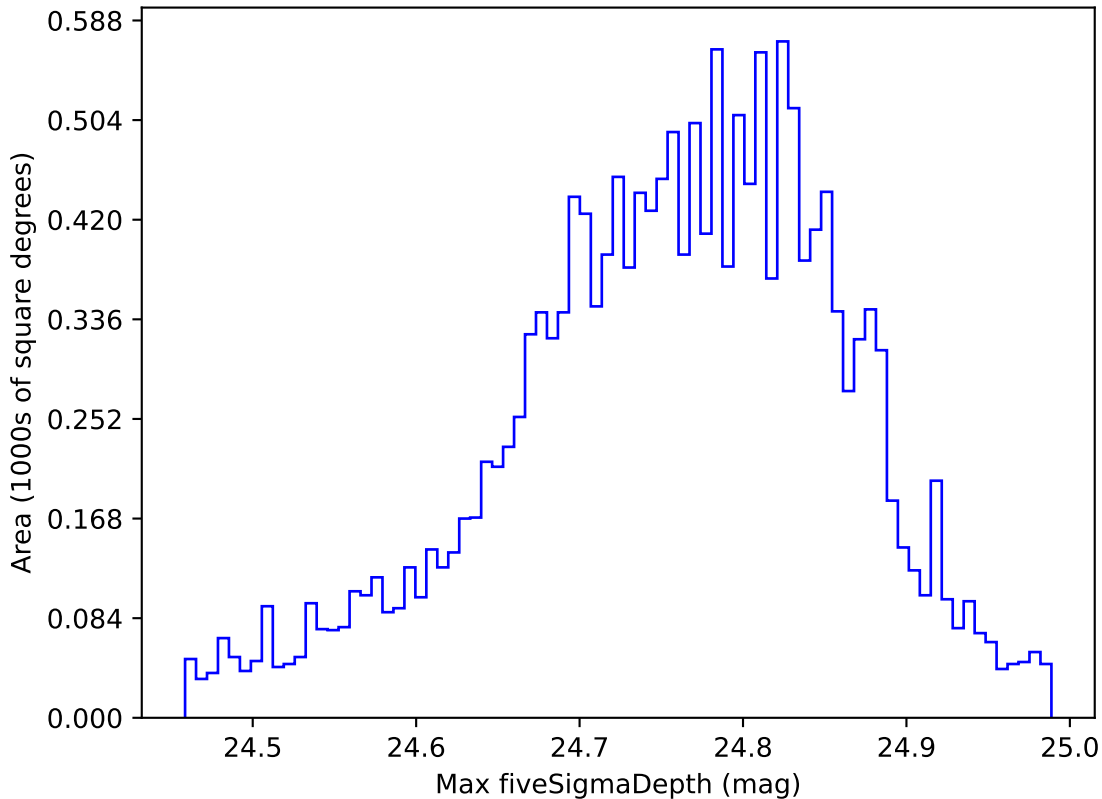
too_elab_r32_d3_griz_v3.4_10yrs WFD r band: Max fiveSigmaDepth
