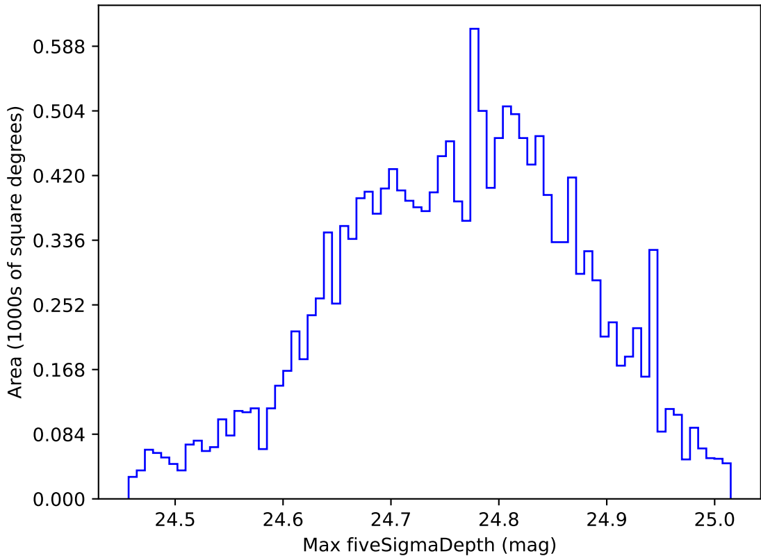
too_elab_r32_d3_griz_v3.4_10yrs WFD r band: Max fiveSigmaDepth
