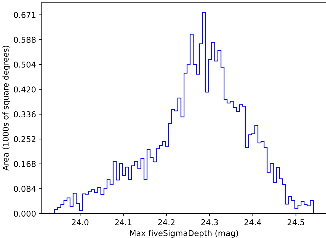
too_elab_r32_d3_griz_v3.4_10yrs WFD i band: Max fiveSigmaDepth
