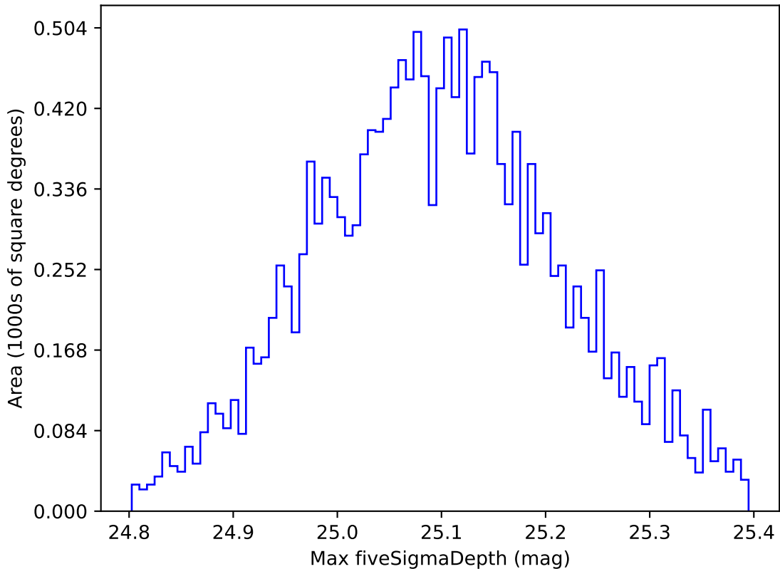
too_elab_r32_d3_griz_v3.4_10yrs WFD g band: Max fiveSigmaDepth
