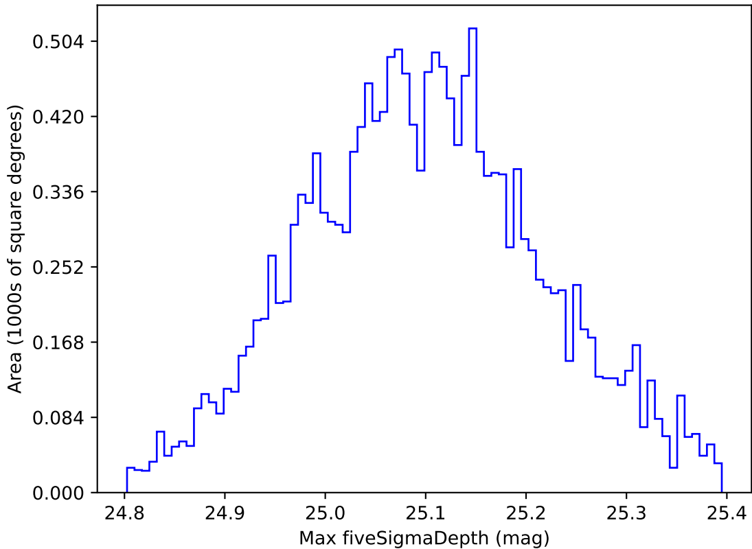
too_elab_r32_d3_griz_v3.4_10yrs WFD all bands: Max fiveSigmaDepth
