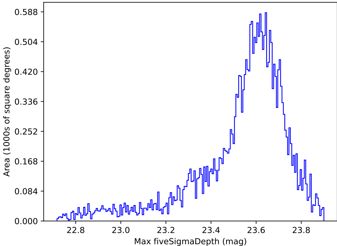
too_elab_r32_d3_griz_v3.4_10yrs All sky z band: Max fiveSigmaDepth
