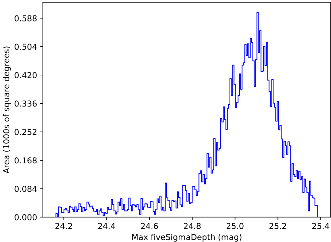
too_elab_r32_d3_griz_v3.4_10yrs All sky g band: Max fiveSigmaDepth
