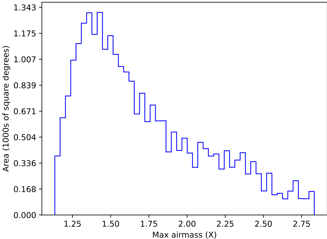
too_elab_r32_d3_griz_v3.4_10yrs Yr 1 z band: Max airmass
