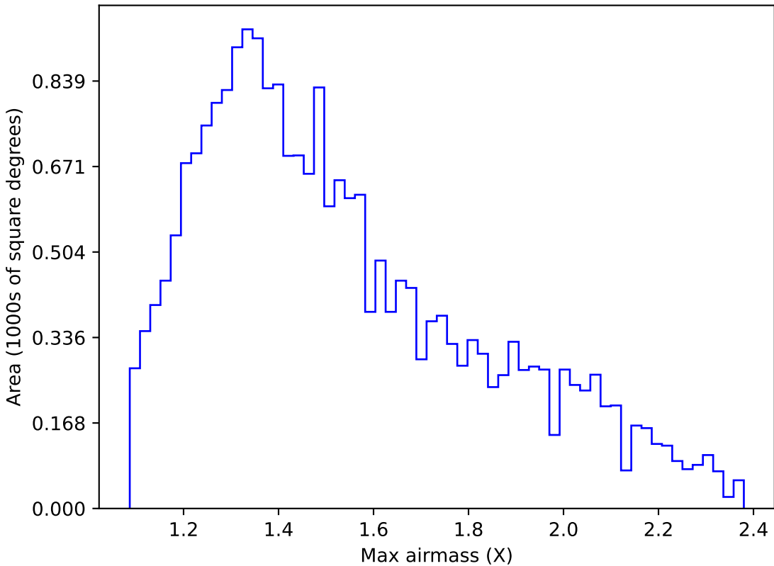
too_elab_r32_d3_griz_v3.4_10yrs Yr 1 u band: Max airmass
