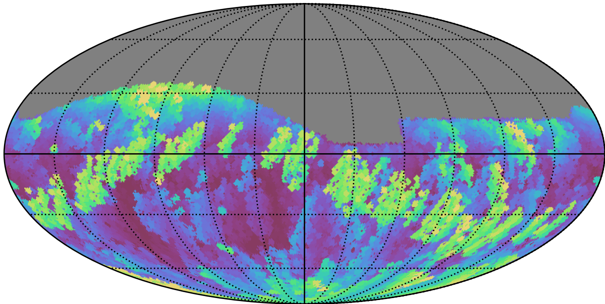
too_elab_r32_d3_griz_v3.4_10yrs Yr 1 r band: Max airmass
