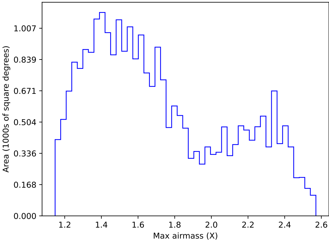
too_elab_r32_d3_griz_v3.4_10yrs Yr 1 r band: Max airmass
