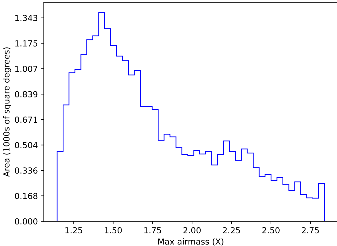
too_elab_r32_d3_griz_v3.4_10yrs Yr 1 i band: Max airmass
