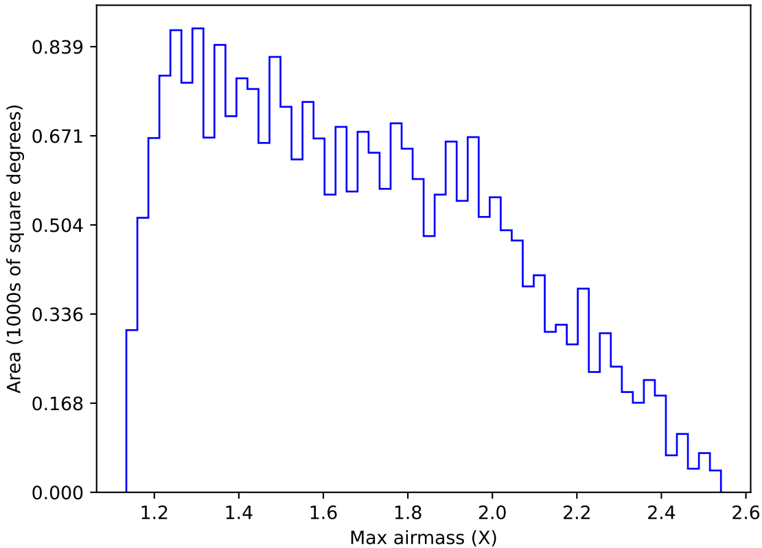
too_elab_r32_d3_griz_v3.4_10yrs Yr 1 g band: Max airmass
