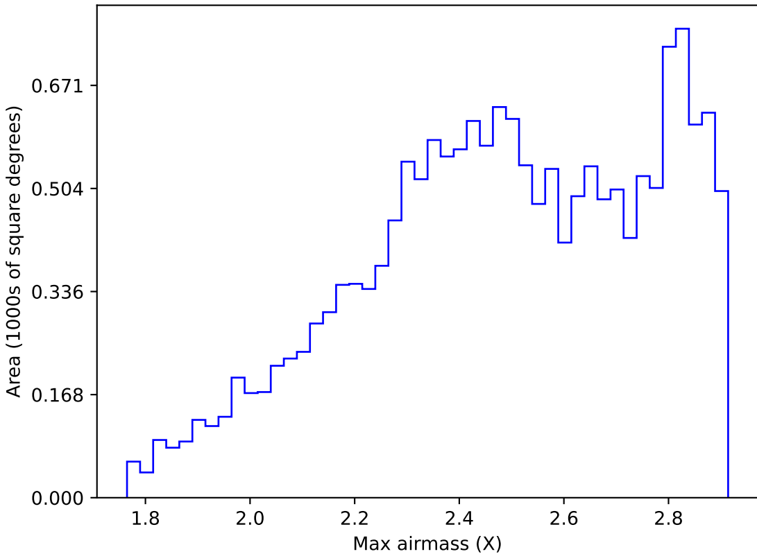
too_elab_r32_d3_griz_v3.4_10yrs WFD z band: Max airmass
