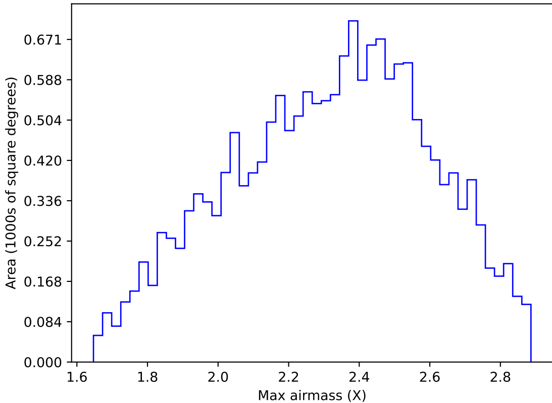
too_elab_r32_d3_griz_v3.4_10yrs WFD y band: Max airmass
