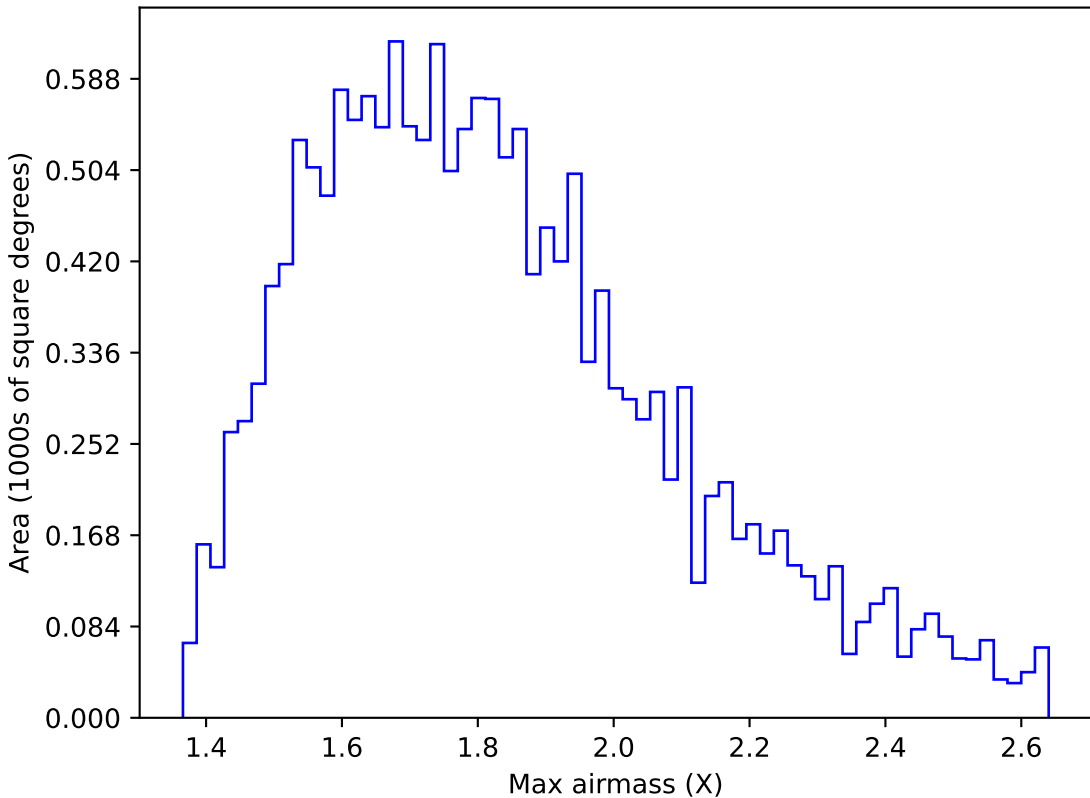
too_elab_r32_d3_griz_v3.4_10yrs WFD u band: Max airmass
