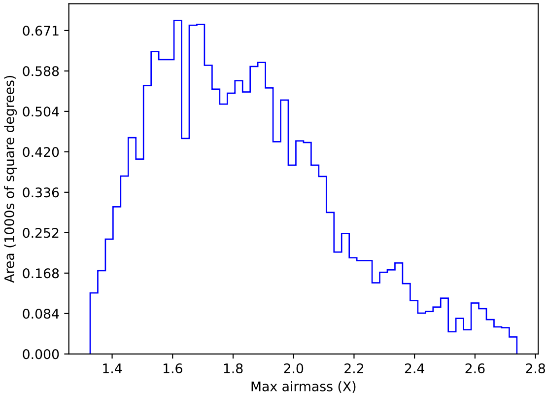
too_elab_r32_d3_griz_v3.4_10yrs WFD u band: Max airmass
