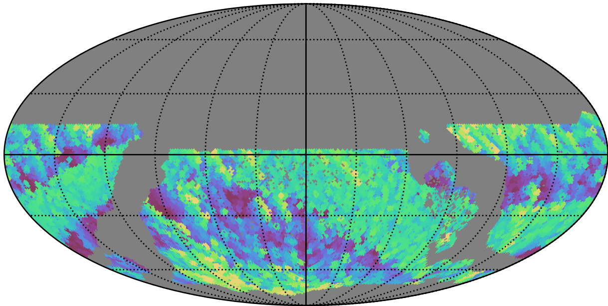
too_elab_r32_d3_griz_v3.4_10yrs WFD r band: Max airmass
