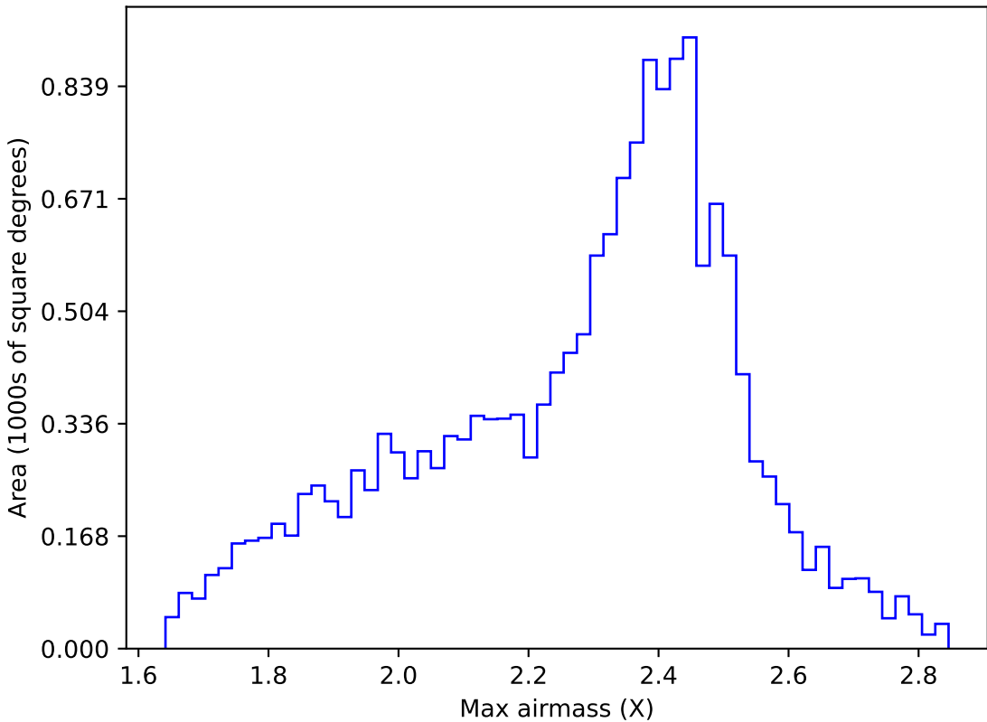
too_elab_r32_d3_griz_v3.4_10yrs WFD r band: Max airmass
