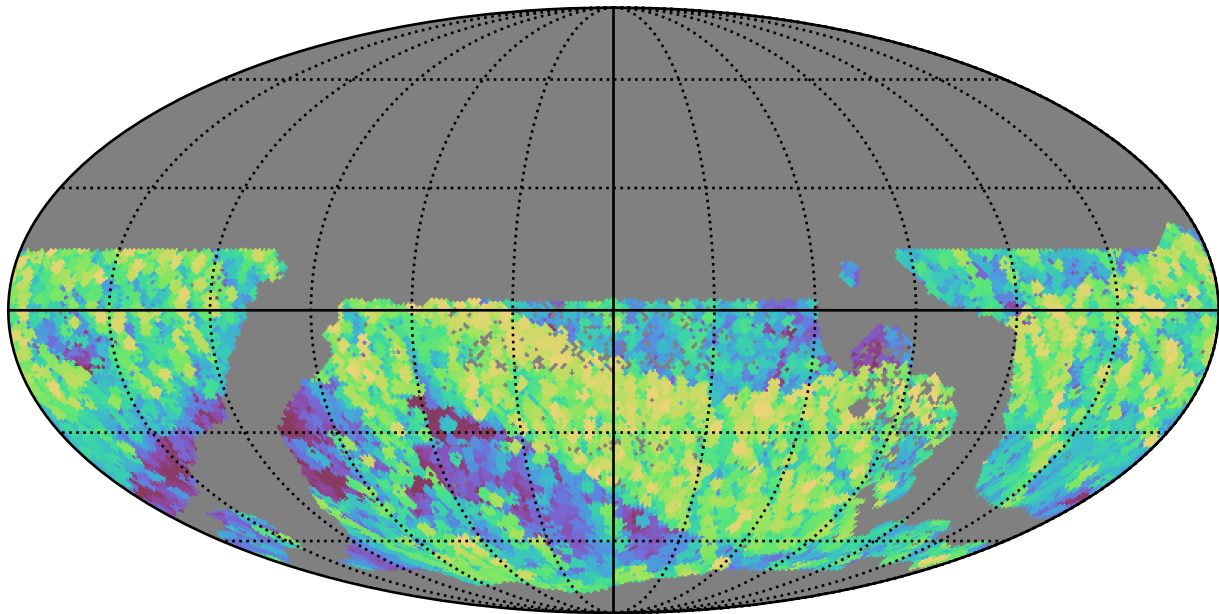
too_elab_r32_d3_griz_v3.4_10yrs WFD i band: Max airmass
