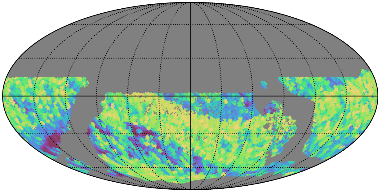
too_elab_r32_d3_griz_v3.4_10yrs WFD all bands: Max airmass
