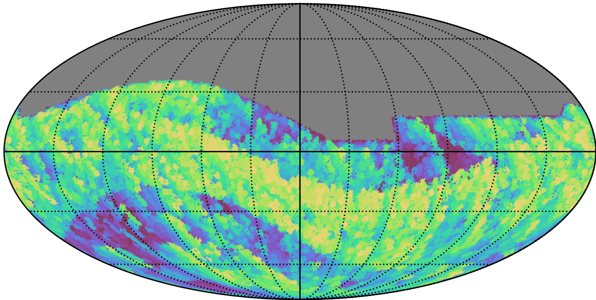
too_elab_r32_d3_griz_v3.4_10yrs All sky z band: Max airmass
