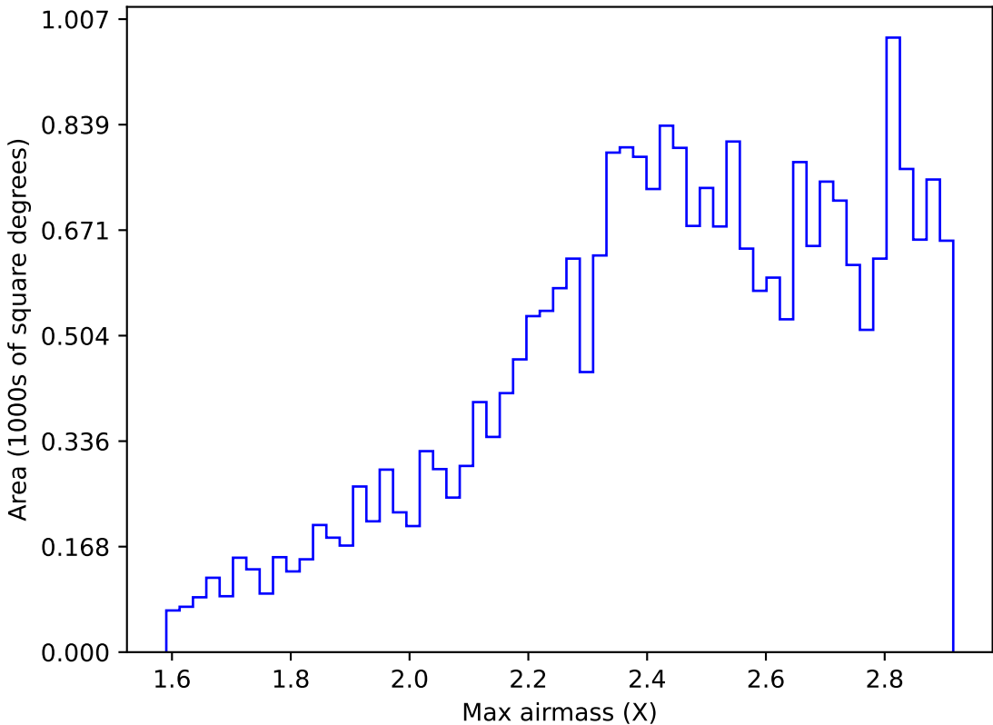
too_elab_r32_d3_griz_v3.4_10yrs All sky z band: Max airmass
